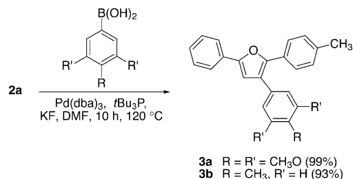
Scheme 2. Suzuki–Miyaura coupling of chlorofuran 2a .
