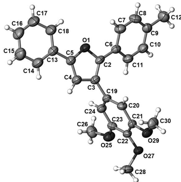
Figure 1. X-ray structure of furan 3a (displacement parameters at the 50% probability level).
