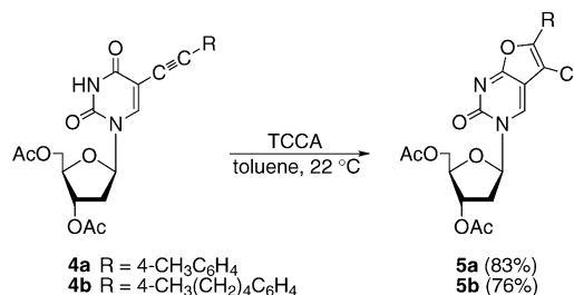
Scheme 3. Synthesis of 5-chlorofuropyrimidine nucleosides 5 .
